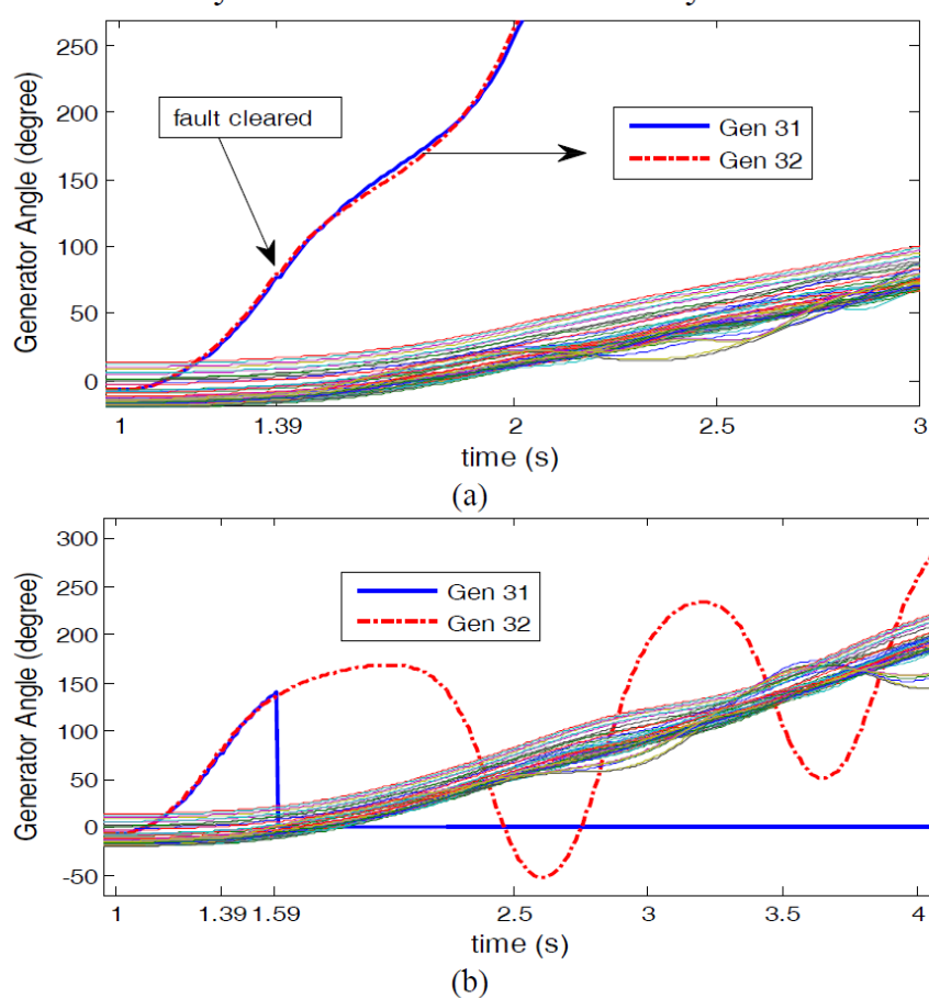
Fig.4: Fault occurs at bus 157 at 1s, cleared at 1.39s. a)no control action, generator 31 (bus 21) and 32 (bus 22) become out of step initially. b)Generator 31 is tripped at 1.59s, system remains stable.
